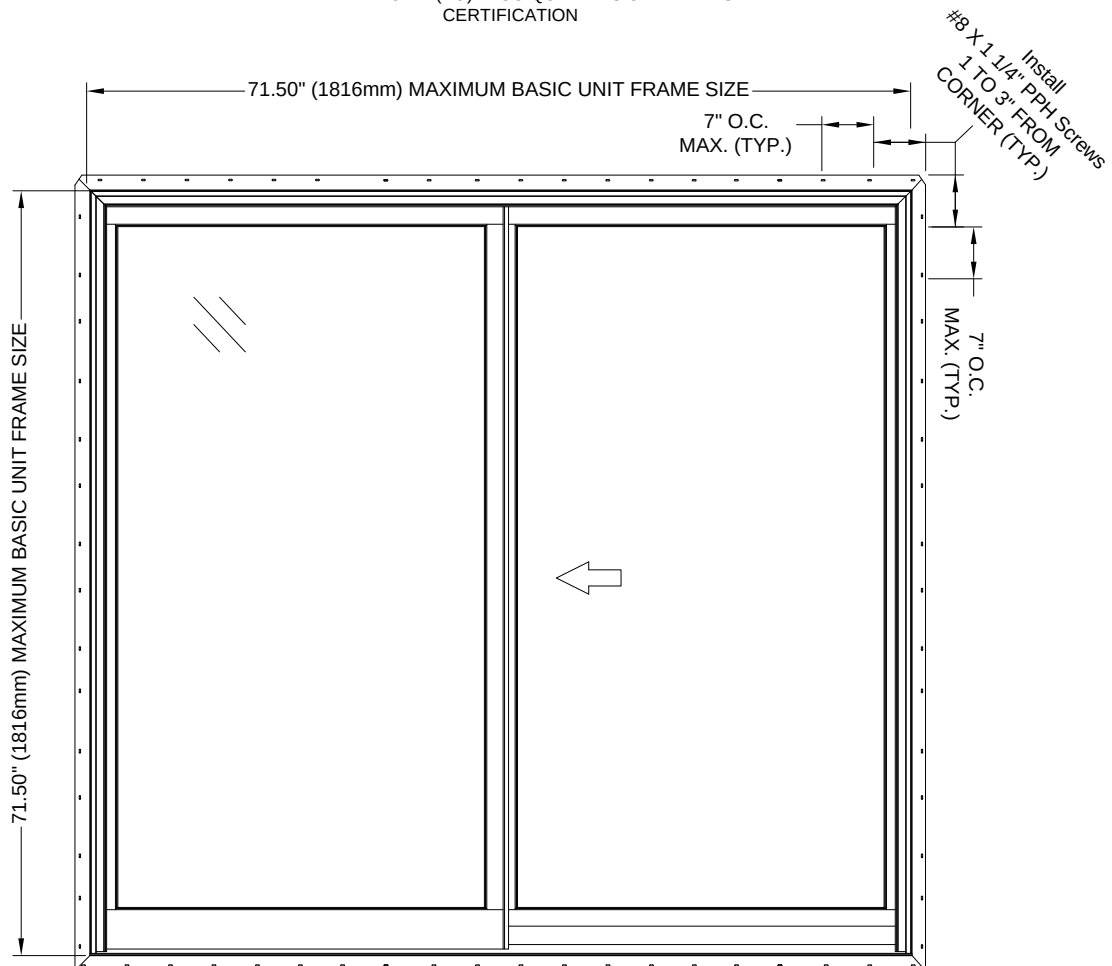
ELEVATION SHOWING FASTENER LOCATION & SPACING VIEWED FROM EXTERIOR
